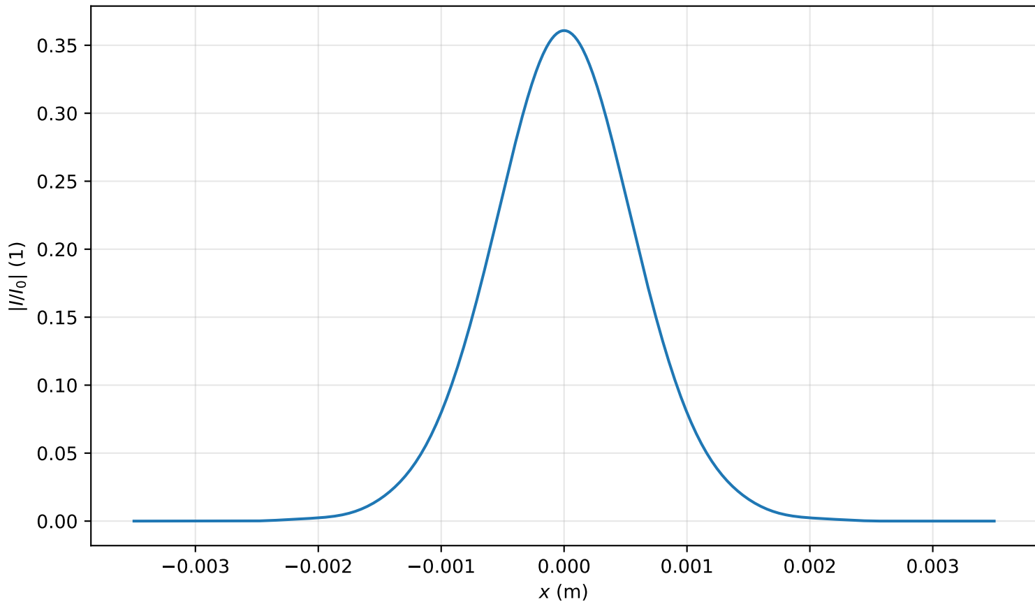
Intensity profile I(x, y = 0, z = 3.742m)/I_0 , P_{in}=0.4P_{cr} , artificial time
